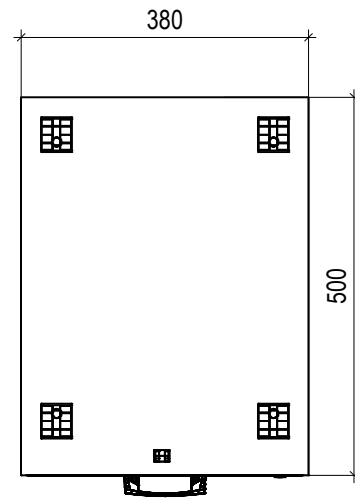
PLAN SCALE 1:10
